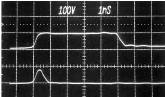
AVR-E4-C-P, at maximum & minimum pulse widths. 100 V/div, 1 ns/div, 100 kHz.
