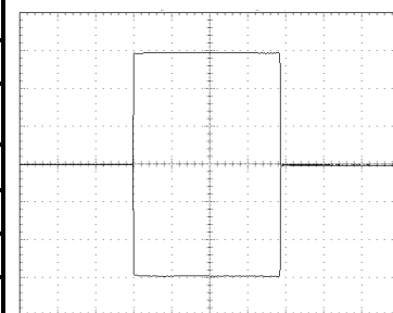
Typical Differential Output, ±950V 2.5μs/Div horizontal scale, 318V/Div vertical scale, center horizontal trace is ground
