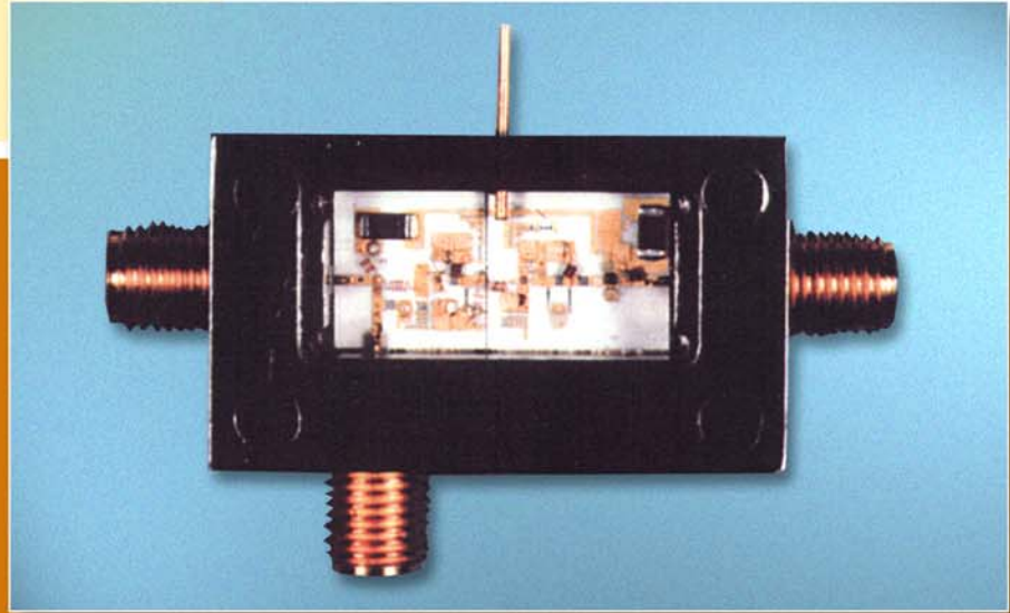
L-BAND LOW NOISE AMPLIFIER Space Qualified - Space Communications
