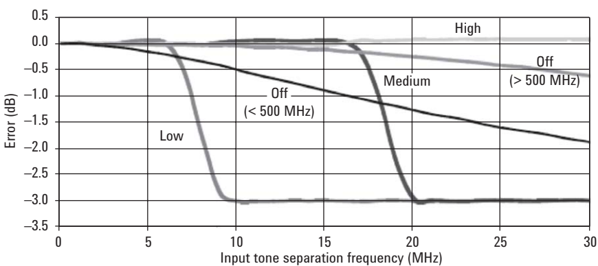
Figure 1. Flatness Response
