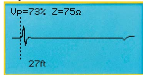
Water Ingress
