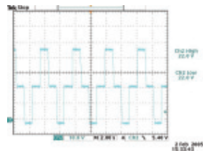
Voltage Step Waveform
