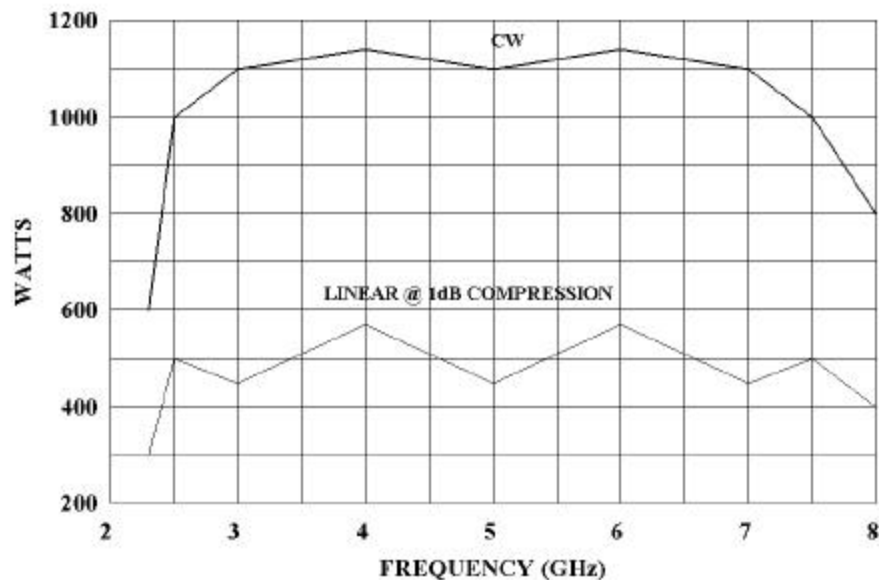
1000T2G8B TYPICAL POWER OUTPUT
