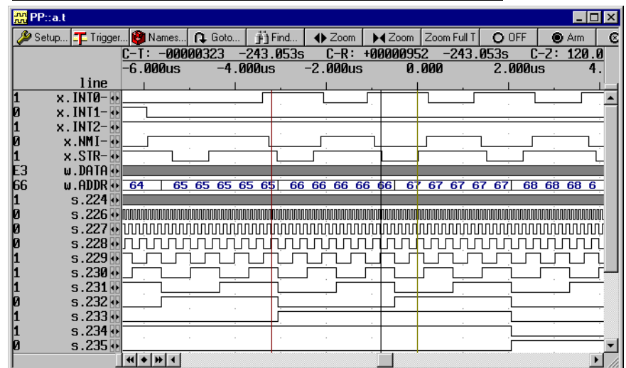
Timing Display
