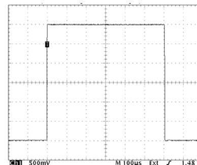
Typical Output Waveform, 3000V (100μs/Div horizontal scale, 500V/Div vertical scale)
