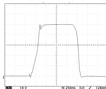
Typical 1μs Output Waveform, 50V 10A (5Ω Load, 250ns/Div Horizontal Scale, 10V/Div Vertical Scale)
